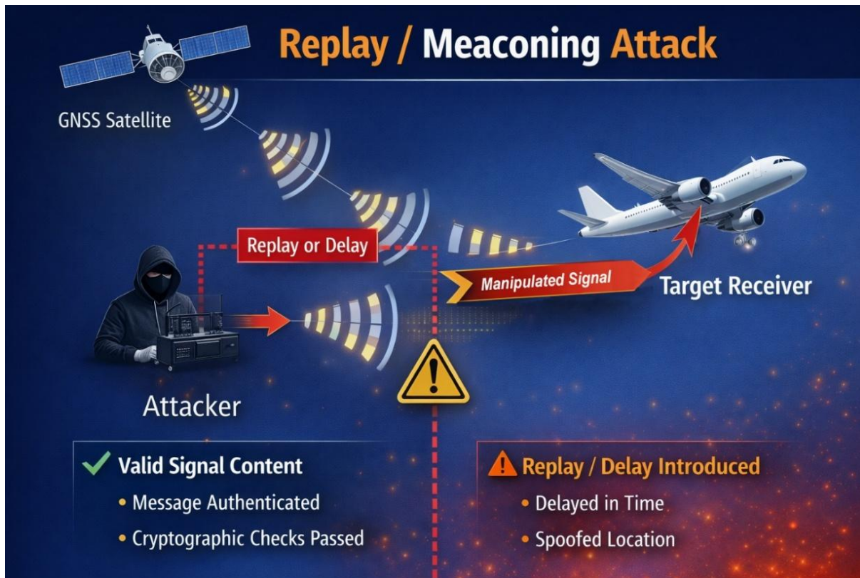
Figure 5. Replay / Meaconing Attack. A delayed rebroadcast of valid navigation signals can preserve message authenticity while altering the receiver's inferred position or timing state.
